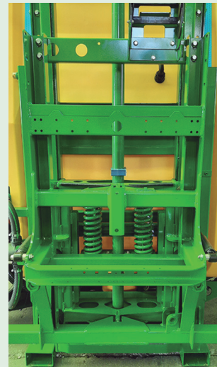
Elevador hidráulico + Suspensión Mecánica. Relevage hydraulique + Suspension mécanique. Hydraulic lift + Mechanical Suspension.
